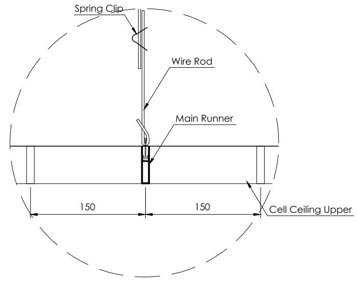
DETAIL 1 SCALE 1:5
