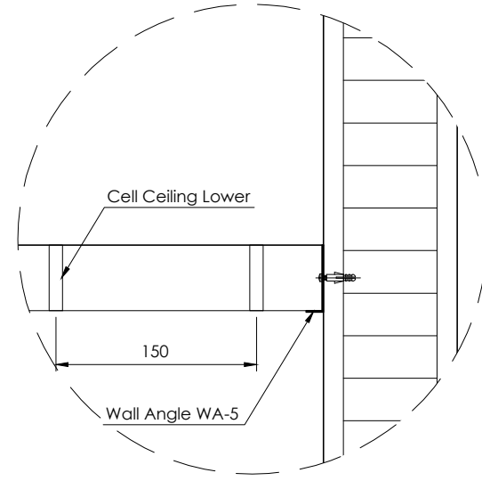
DETAIL 2 SCALE 1:5
